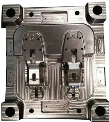
Cavity Plate
